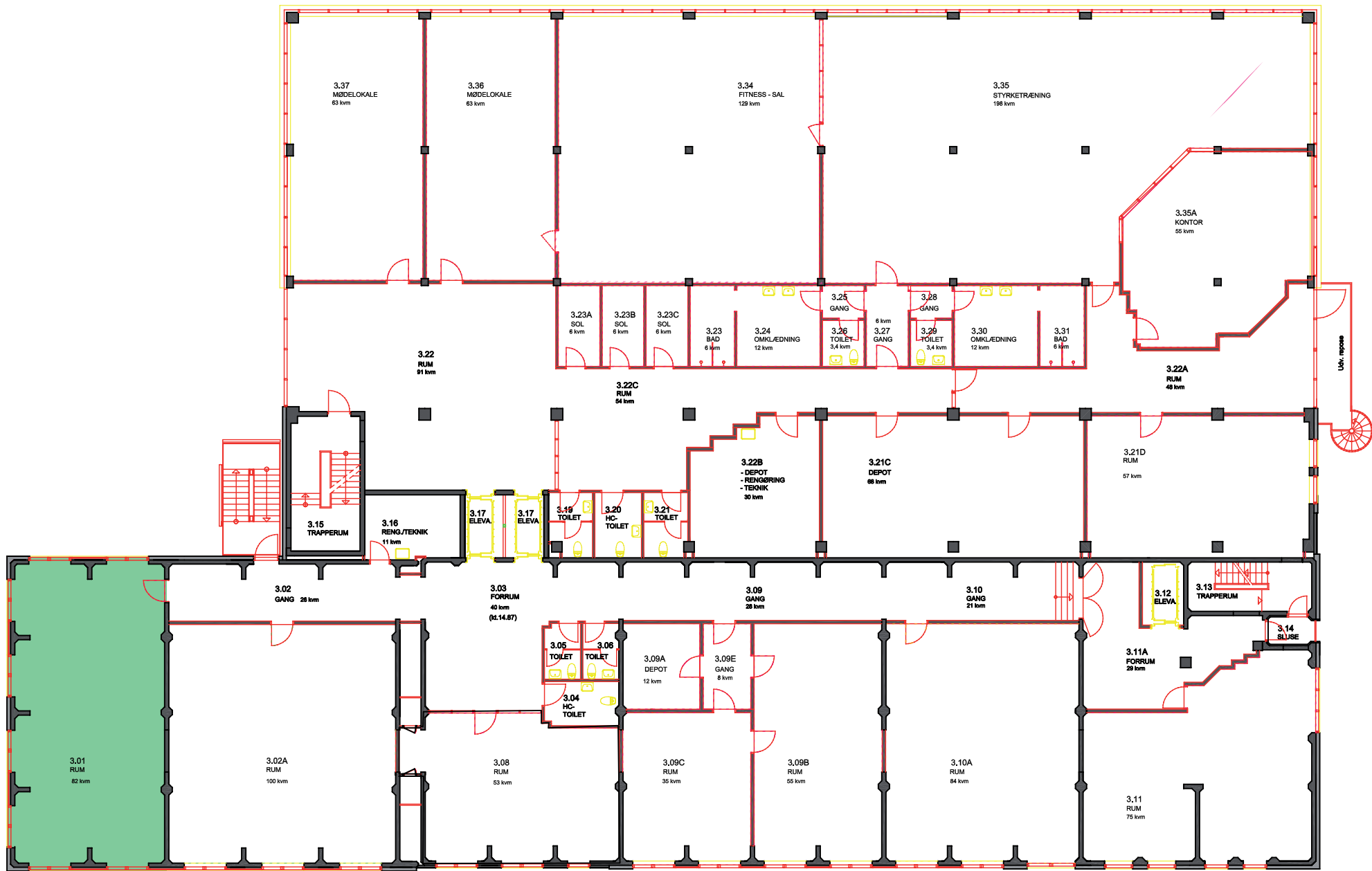
KATTEGAT SILO 3. SALS PLAN
